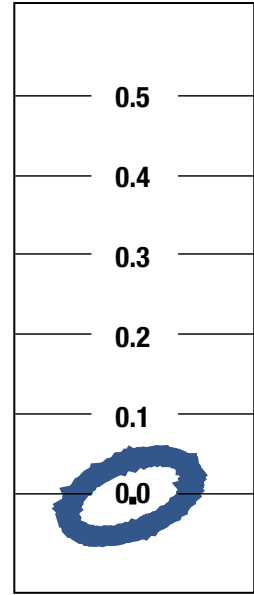
METALS (ppm)
